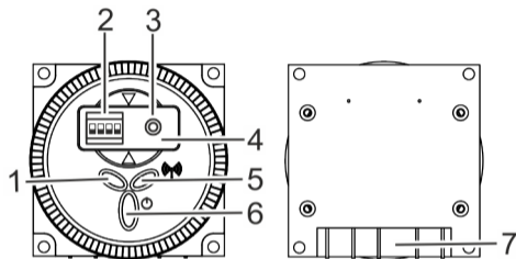
Fig. 2: Overview of actuator (receiver) "RecFM/2"
